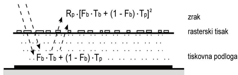
Slika 13. Yule-Nielsenov model
