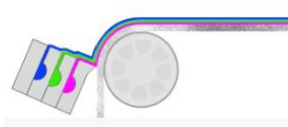
Figure 13 - Slide Bead Coating
