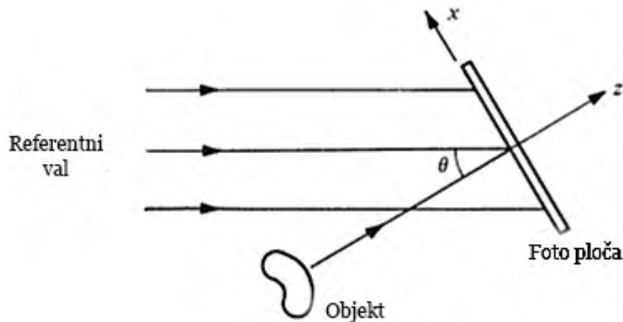
Shema 7. Snimanje holograma off axis
