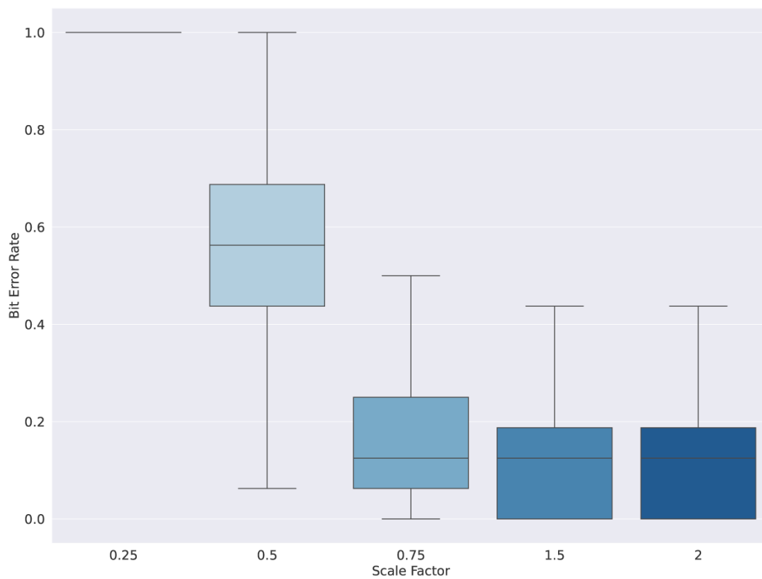
Figure 22. Boxplots displaying BER values for images after scaling.
