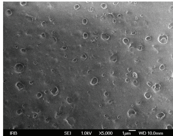
» Figure 8: SEM micrograph of green thermochromic print after interaction with ethanol (magnification 5000x)
