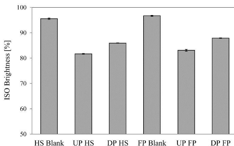
Figure 3. Brightness of blank samples and undeinked (UP) and deinked (DP) pulps
