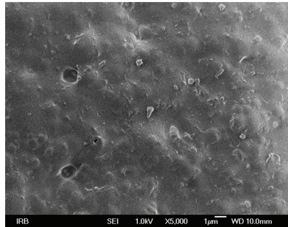
» Figure 6: SEM micrograph of green thermochromic print after interaction with acetone (magnification 5000x)
