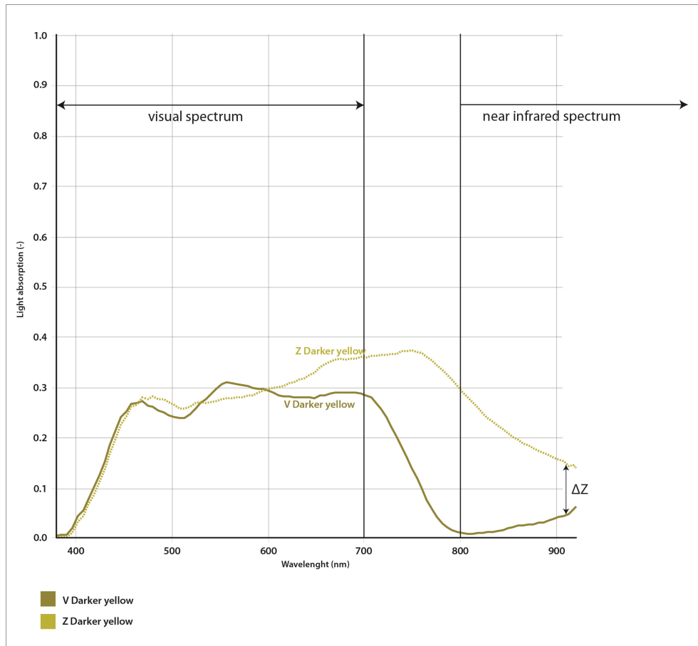
Chart 5. Spectrogram color twin dyes called: Darker yellow; \Delta E = 3,54 (Table 17.)
