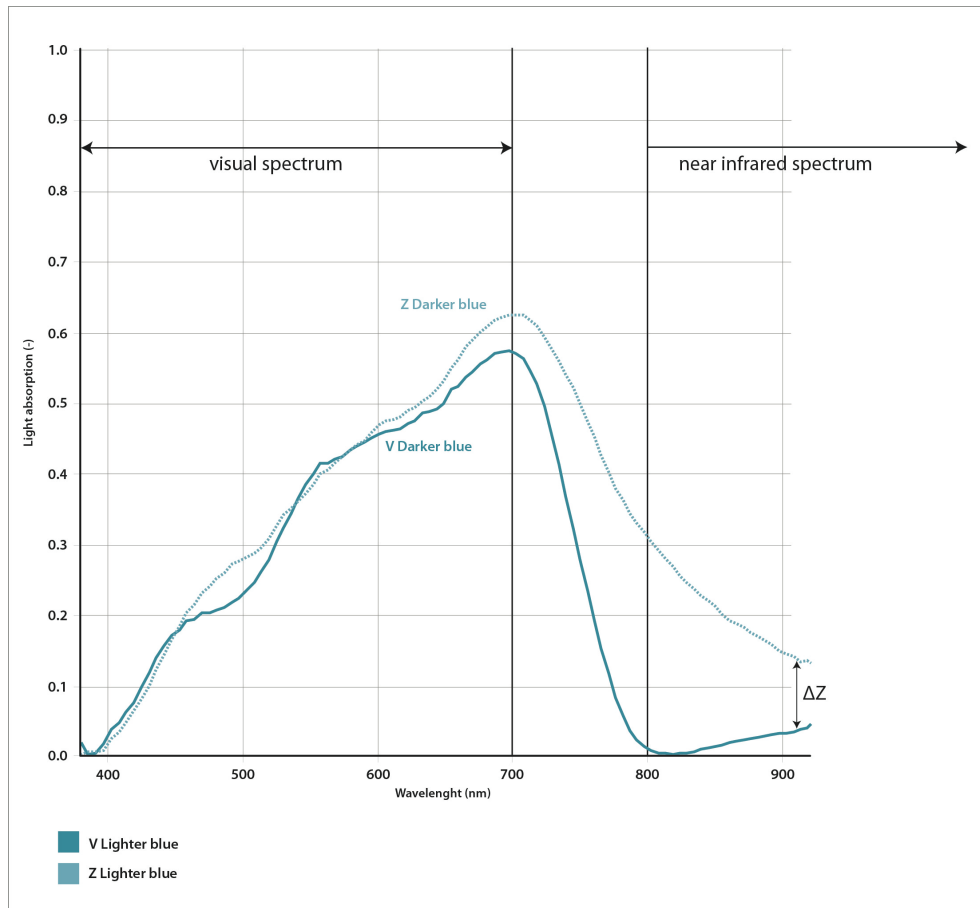
Chart 2. Spectrogram color twin dyes called: Lighter blue; \Delta E = 2,73 (Table 17.)
