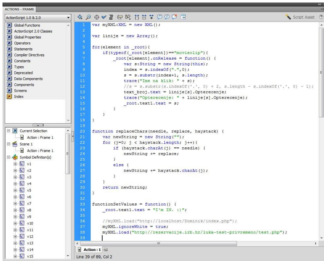
Slika 23: ActionScript.
