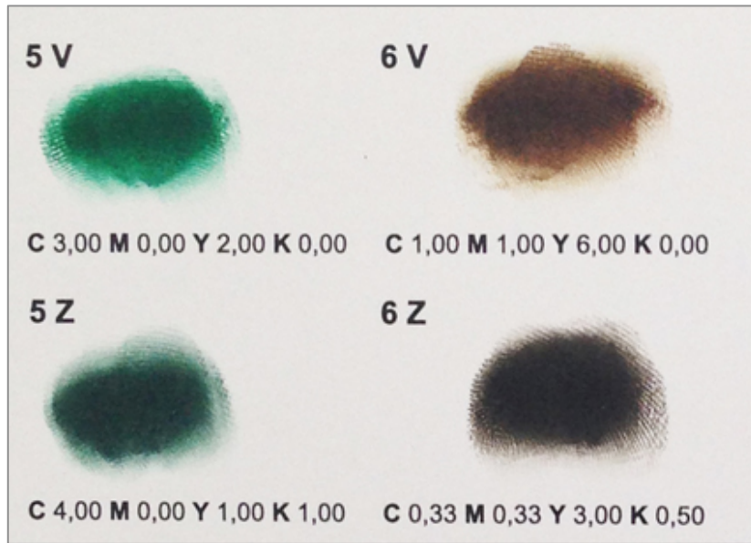
Figure 48. Dye twins for offset printing in the visual spectrum, twin dyes 5V, 5Z and 6V, 6Z
