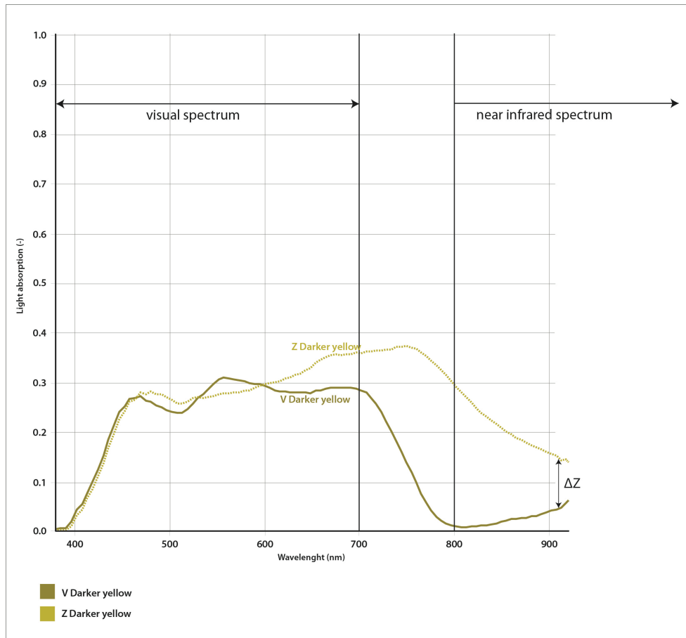
Chart 5. Spectrogram color twin dyes called: Darker yellow; \Delta E = 3,54 (Table 17.)
