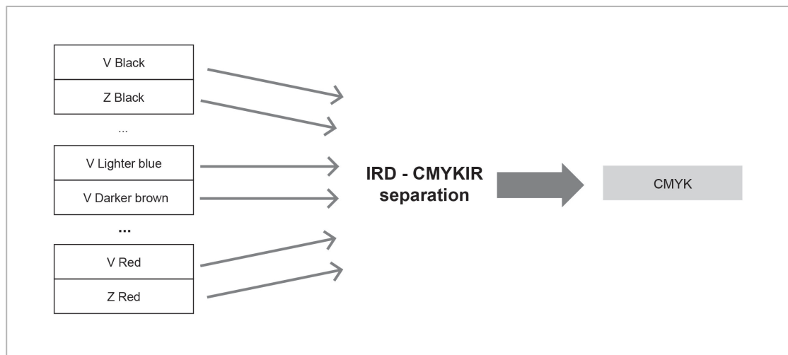
Figure 61. Process of CMYKIR separation in infrared mapping
