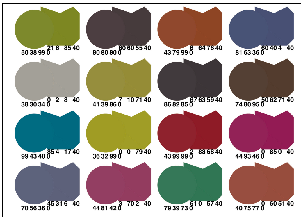
Figure 6. Twin dyes with the same visual experience but different NIR response
