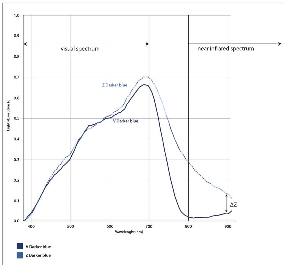
Chart 1. Spectrogram color twin dyes named: Darker blue; \Delta E = 3,85 (Table 17.)
