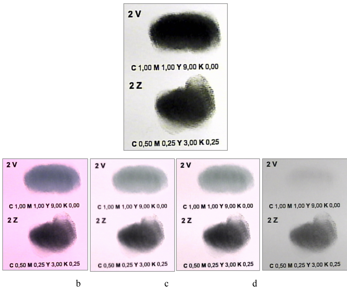
Figure 52. Display of barrier cuts at 570nm, 695nm, 715nm and 850nm of twin dyes 2V and 2Z
