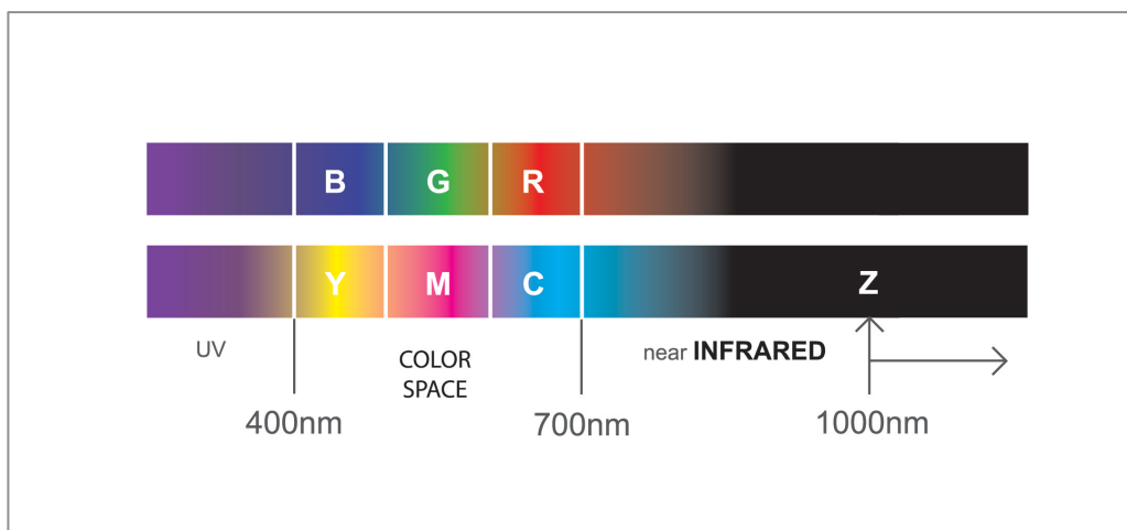
Figure 1. The visual range (V) of 400 to 700nm RGB and CMYK color space visible to the naked eye and near infrared (NIR) range from 750 to 1000nm not visible to the naked eye.
