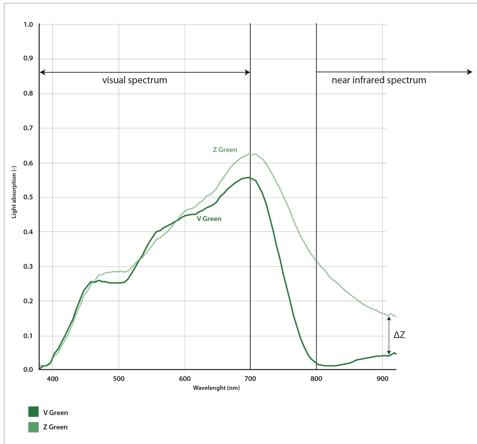
Chart 3. Spectrogram color twin dyes called: Green; \Delta E = 2,13 (Table 17.)
