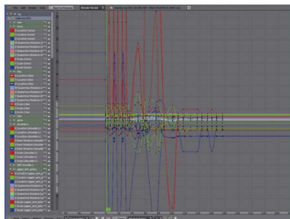
Slika 64: Graph editor
