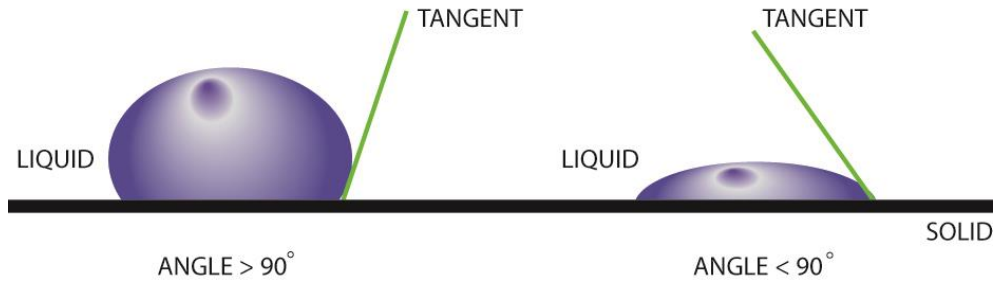
Figure 26 Schematic representation of contact angle
