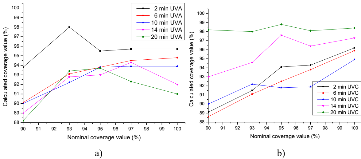
Figure 71. Changes in high coverage area on prints obtained by UV post-treated Digital MAX printing plates:
