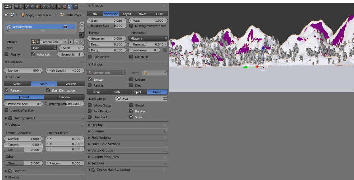
Slika 18: Particle system
