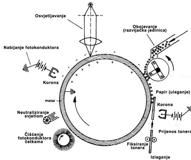
Slika 4. Osnovni princip elektrofotografije (Izvor: http://what-when-how.com/electronic-properties-of-materials/electrical-properties-of-polymers-ceramics-dielectrics-and-amorphous-materials-part-2/ )
